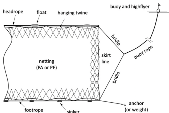
Set gillnet – main components
